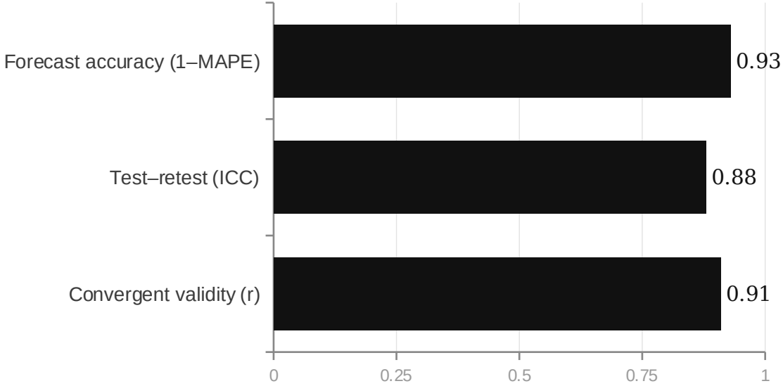
ABILITYSCORE® — VALIDATION
